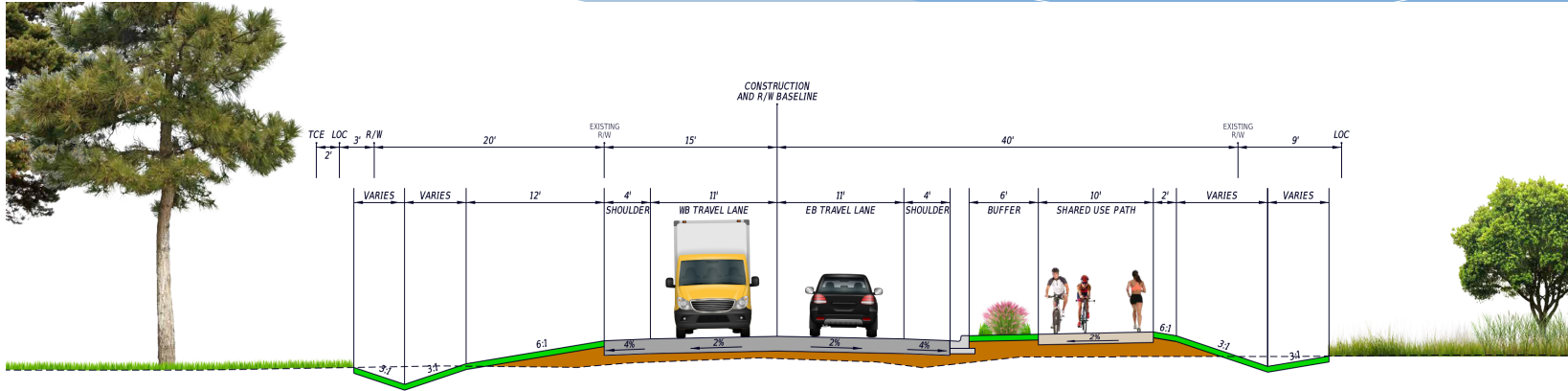
TYPICAL SECTION 1: SCHAFFER LANE LOOKING EAST TOWARD BRIDGE
