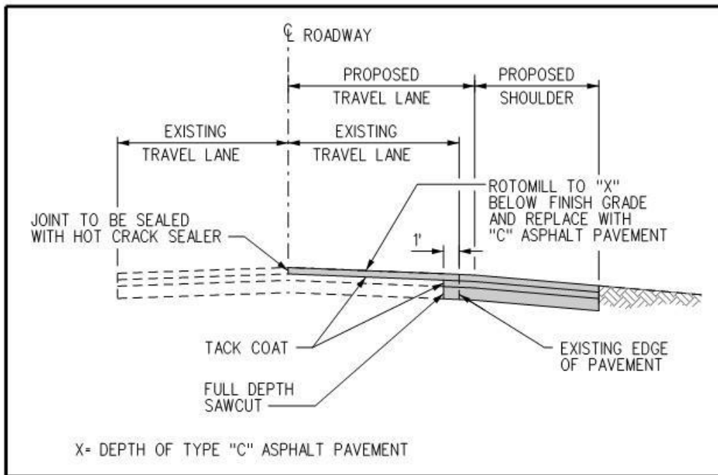
Figure 5.6.4-b Lane Widening/Restoration Detail
