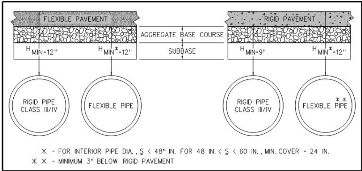
Figure 5.7.2.5-b Existing Pavement Shallow Pipe Cover Details
