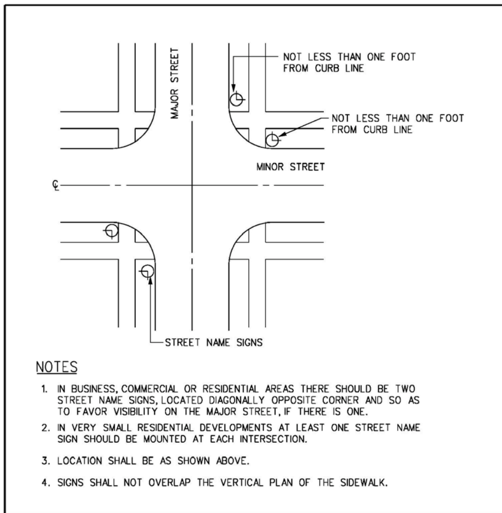
Figure 5.11.1.3-a Street Name Sign Location
