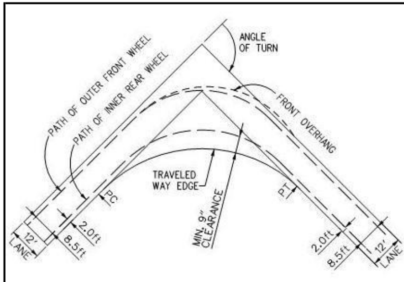
Figure 5.2.5.6-a Turning Movement Offsets
