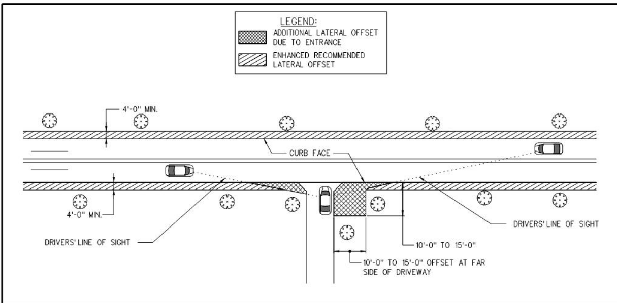
Figure 5.5.6-c Lateral Offsets at Entrances
