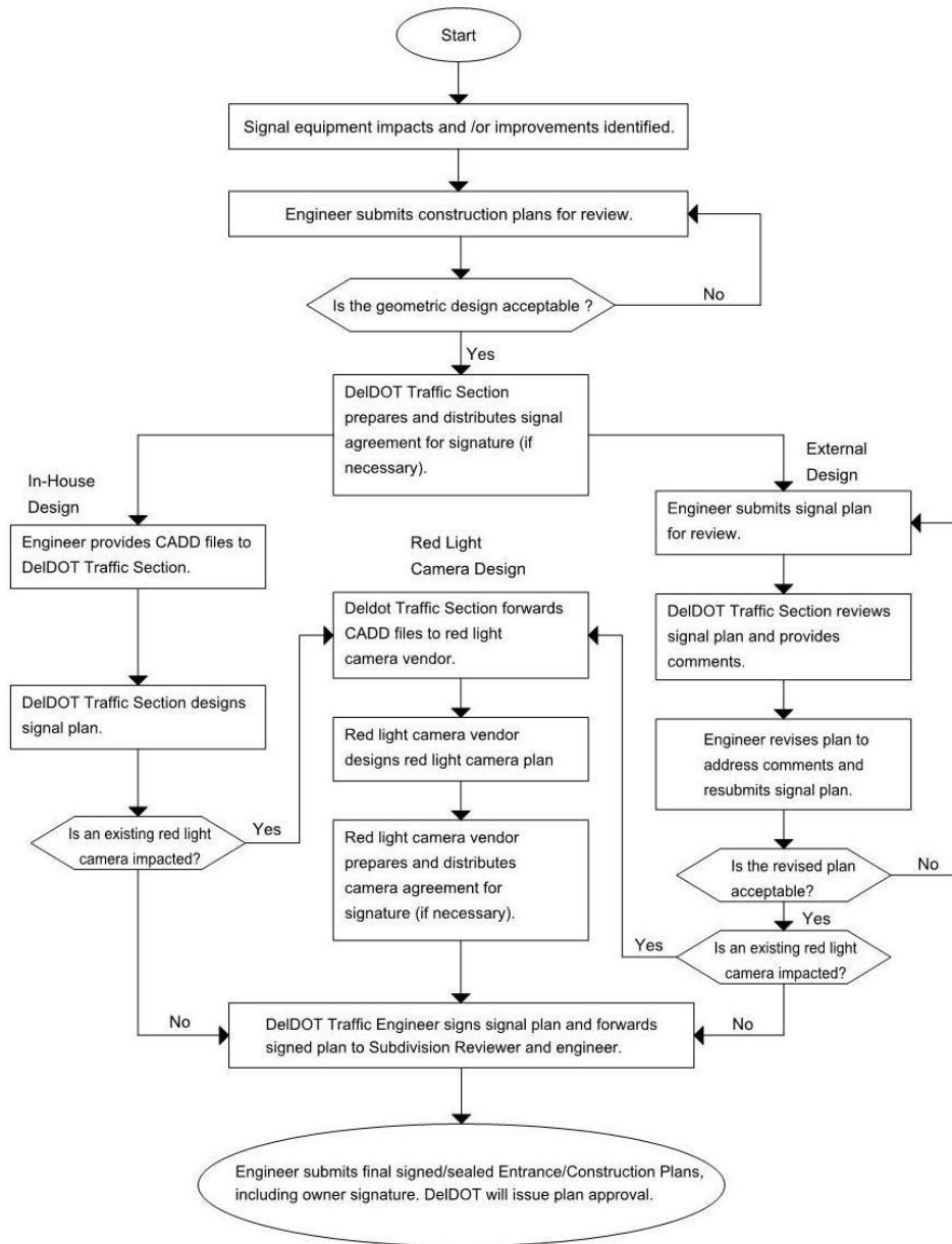
Figure 5.13-a Signal Design Flow Chart
