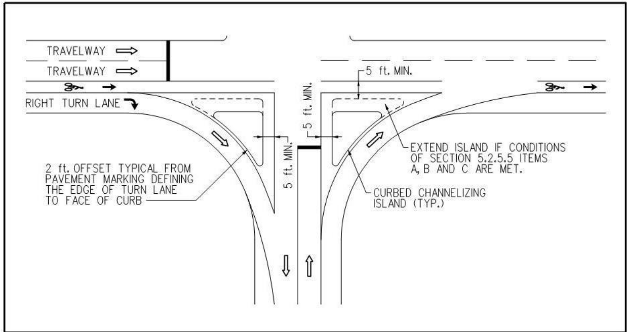
Figure 5.2.5.5-c Triangular Island Offsets
