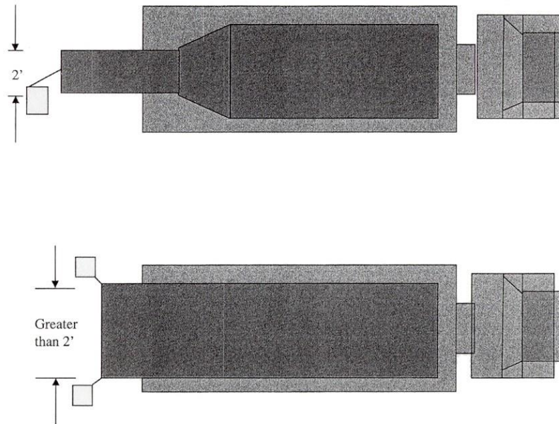
Figure 4.2: Warning Flaps on Overlength Loads or Loads With a Rear-End Overhang Source: AASHTO Guide for Vehicle Weights and Dimensions
