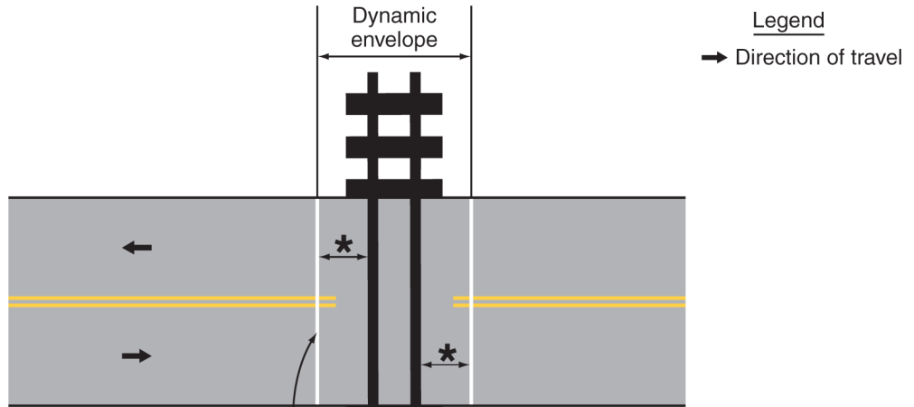
Figure 8B-8. Example of Dynamic Envelope Pavement Markings at Grade Crossings
