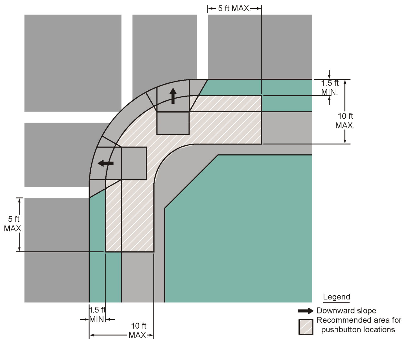
Figure 4E-3. Pushbutton Location Area (Delaware Revision)
