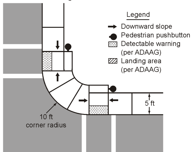
C - Parallel ramps with narrow sidewalk and tight corner radius
