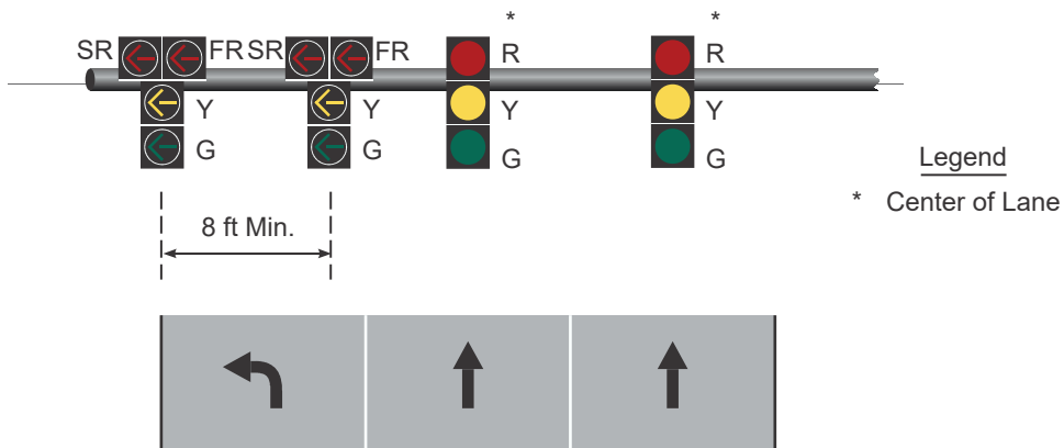
Figure IV-5e. Two Through Lanes with One Left-Turn Lane (Protected-Permissive Left-Turn Phasing FRA)
