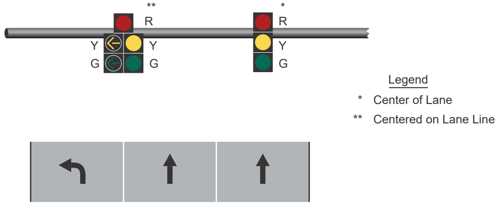
Figure IV-5d. Two Through Lanes with One Left-Turn Lane (Protected-Permissive Left-Turn Phasing)
