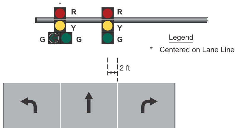
Figure IV-6d. One Left-Turn Lane, One Through Lane, and One Right-Turn Lane (Split Phasing)
