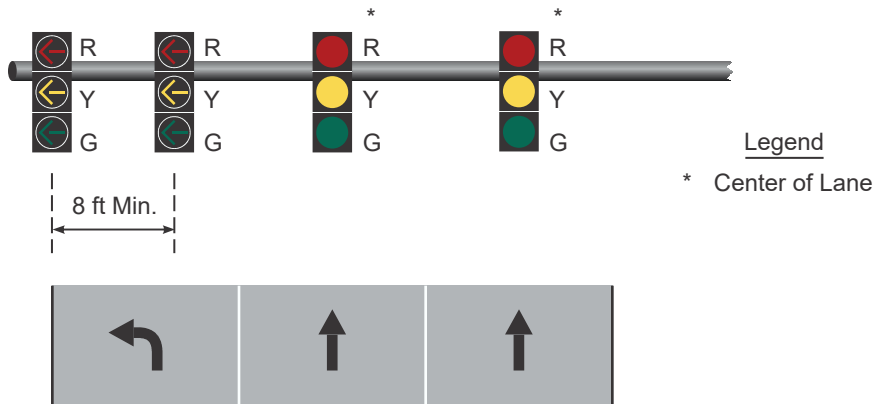
Figure IV-5f. Two Through Lanes with One Left-Turn Lane (Protected-Only Left-Turn Phasing)
