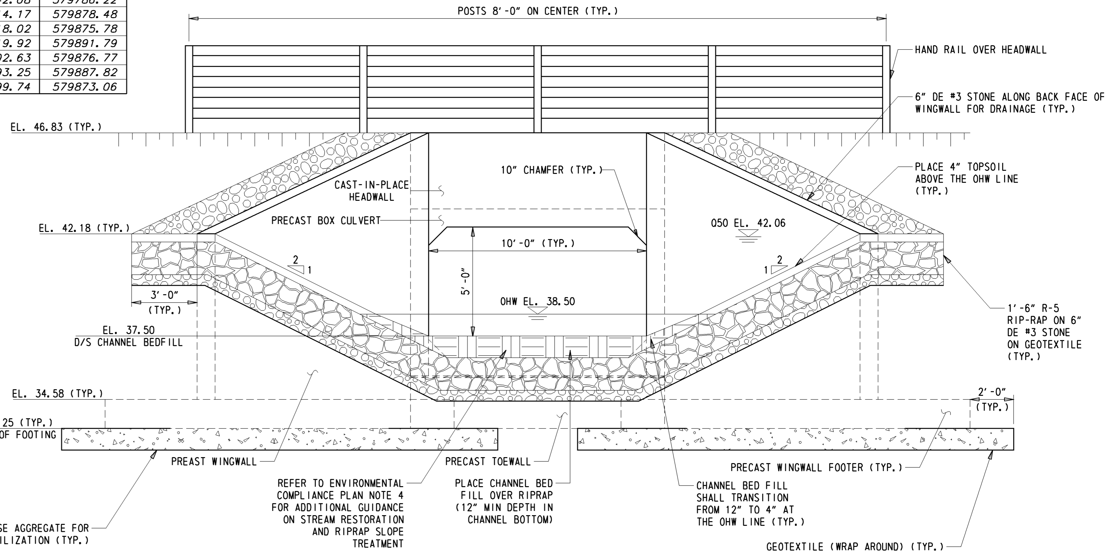
TYPICAL ELEVATION 3/8" = 1'-0"
