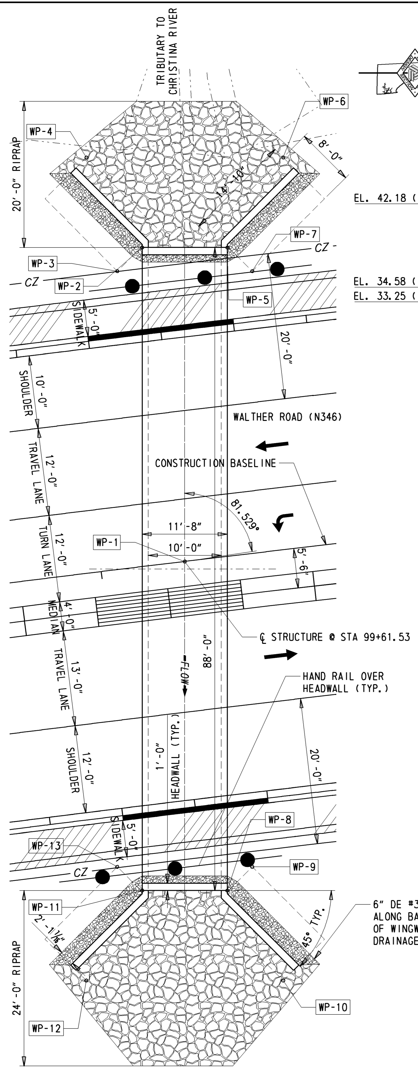
PLAN 1/8" = 1'-0"
