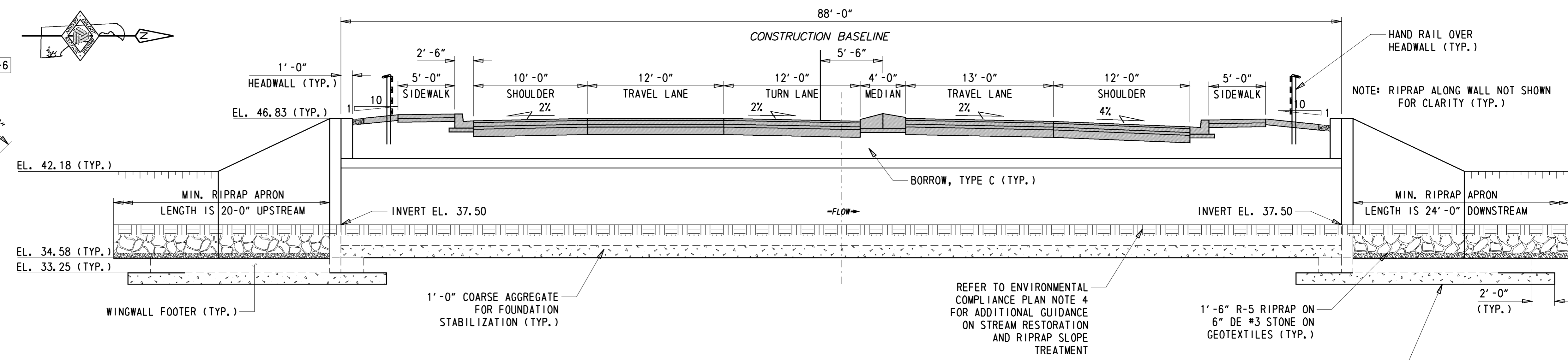
TYPICAL SECTION 3/16" = 1'-0"
