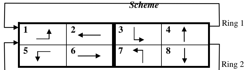
Figure P-1 Typical Phase numbering
