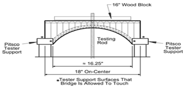
Figure 3. Tester Configuration Detail
