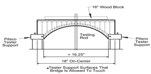
Figure 3. Tester Configuration Detail
