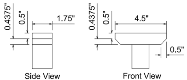
Figure 4. Support Detail
