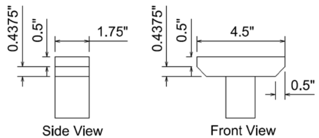
Figure 4. Support Detail
