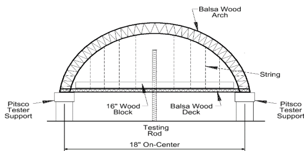
Figure 3. Tester Configuration Detail
