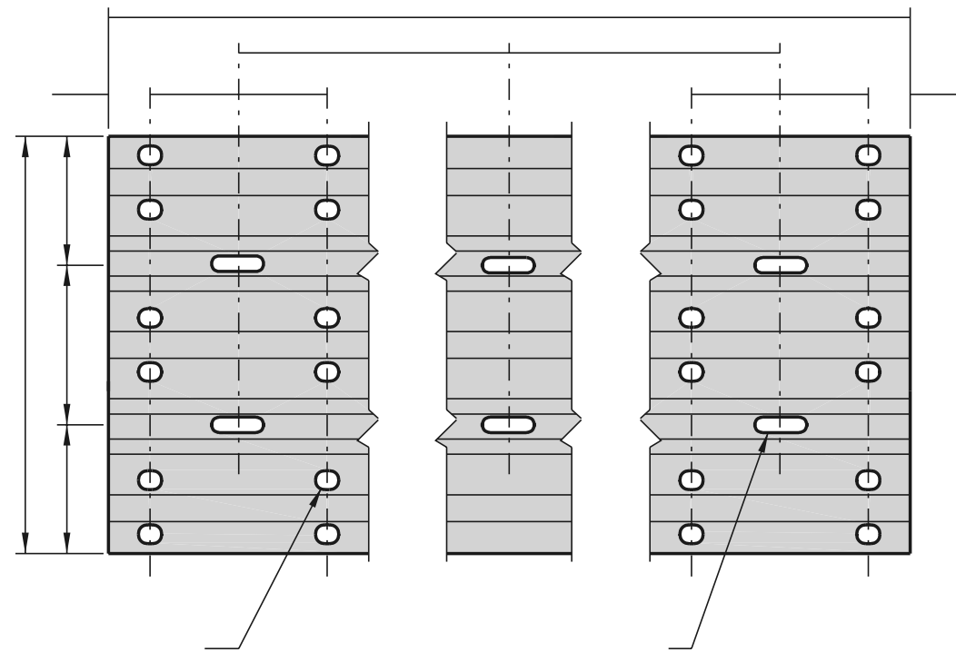
THRIE BEAM ELEVATION
