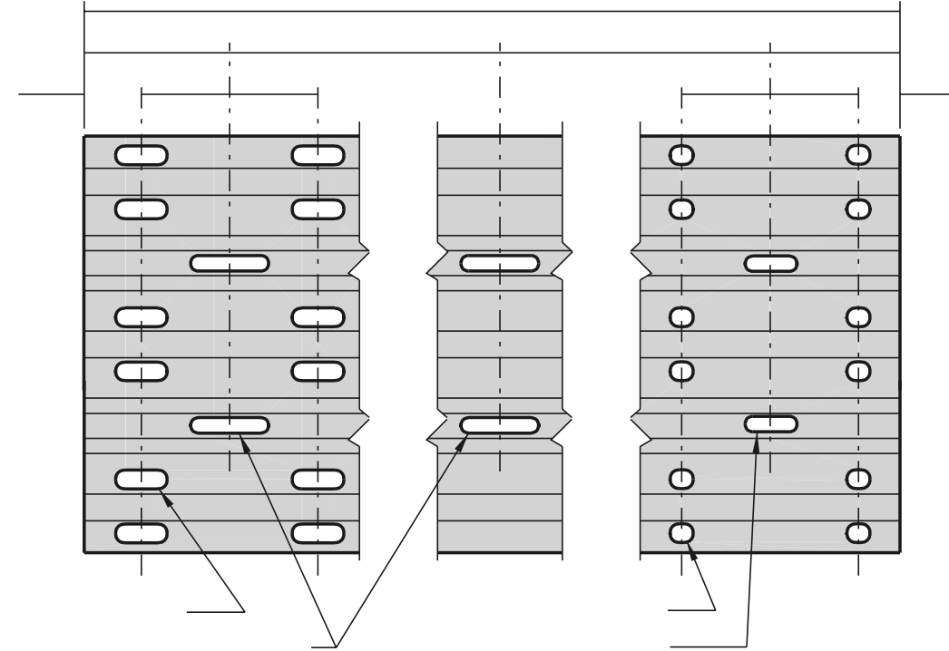
THRIE BEAM EXPANSION ELEMENT
