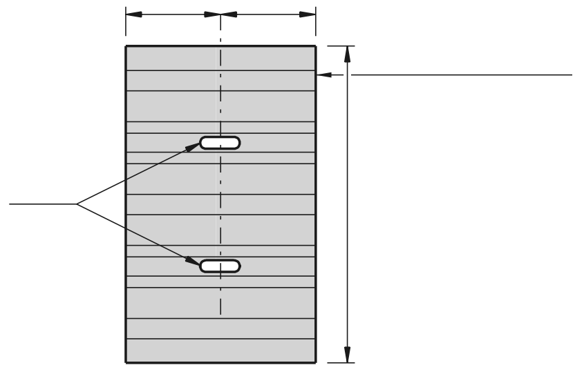
THRIE BEAM BACK-UP PLATE (SAME SECTION AS THRIE BEAM)
