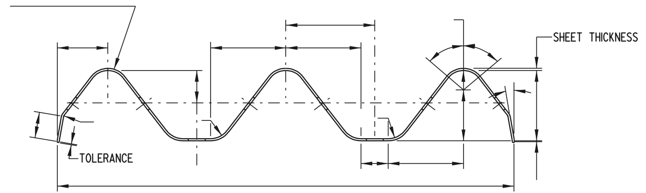
THRIE BEAM SECTION
