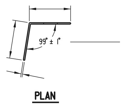
REFLECTORIZED WASHER
