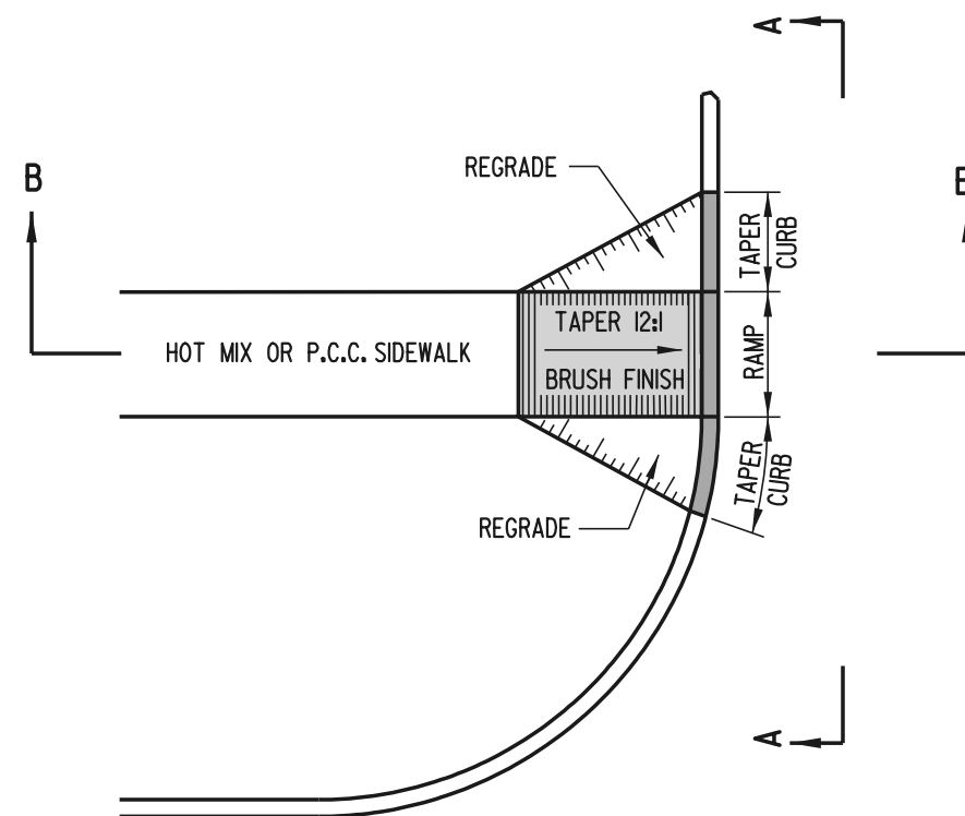
CURB RAMP, TYPE I
