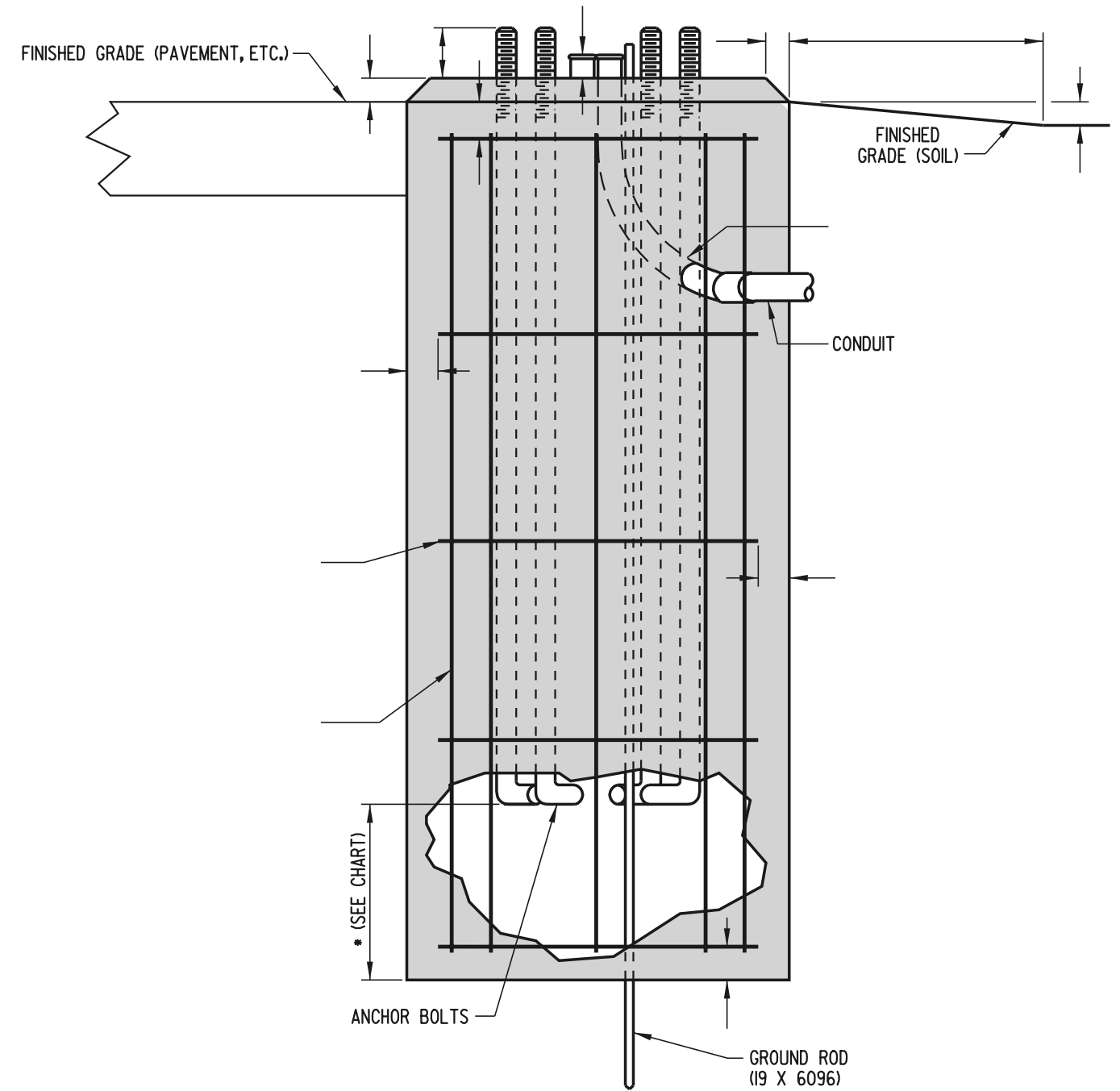
TYPICAL SECTION (BASES 5 AND 6)
