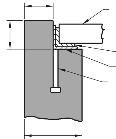
FRAME & GRATE ASSEMBLY DETAIL
