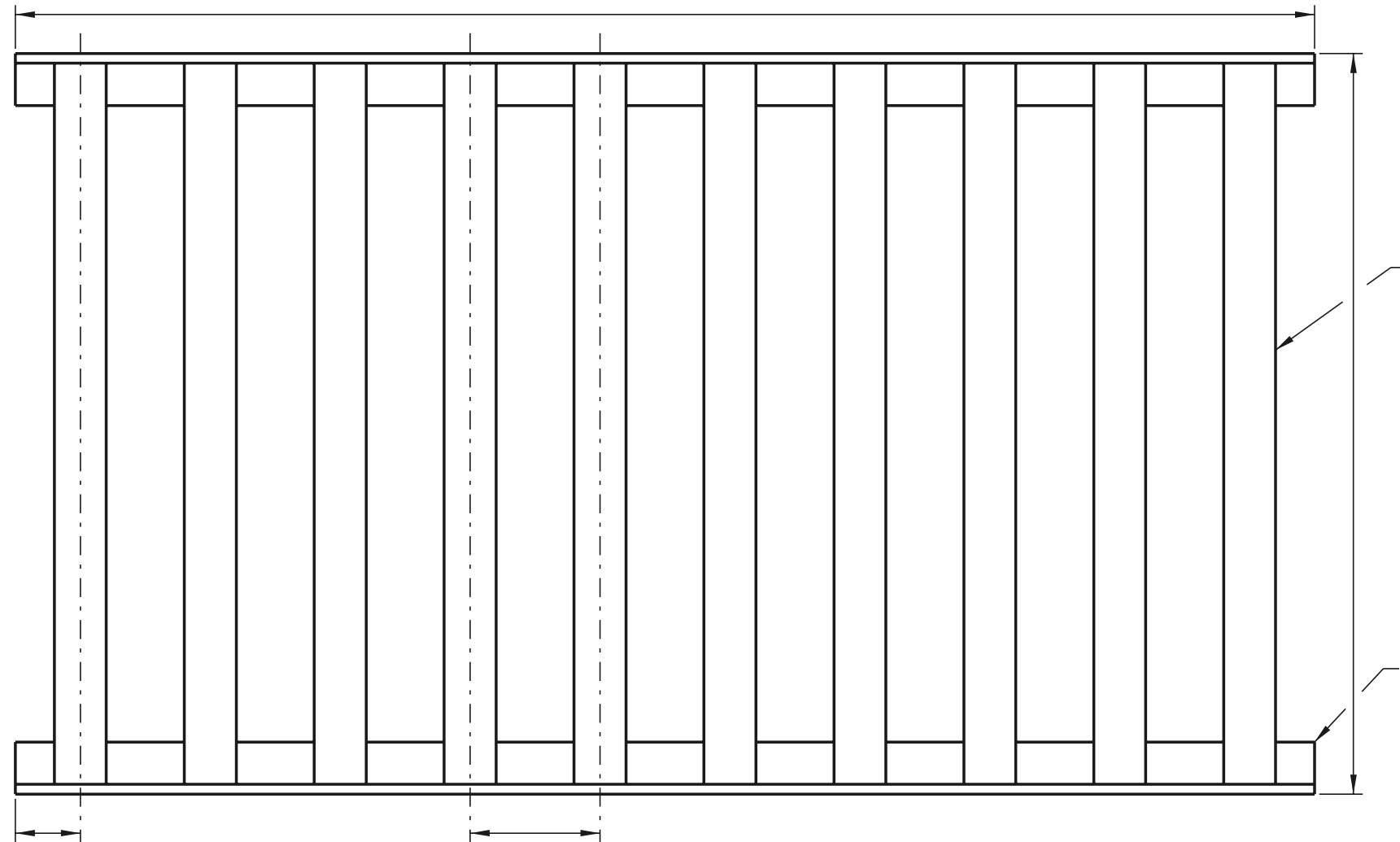
GRATE DETAIL
