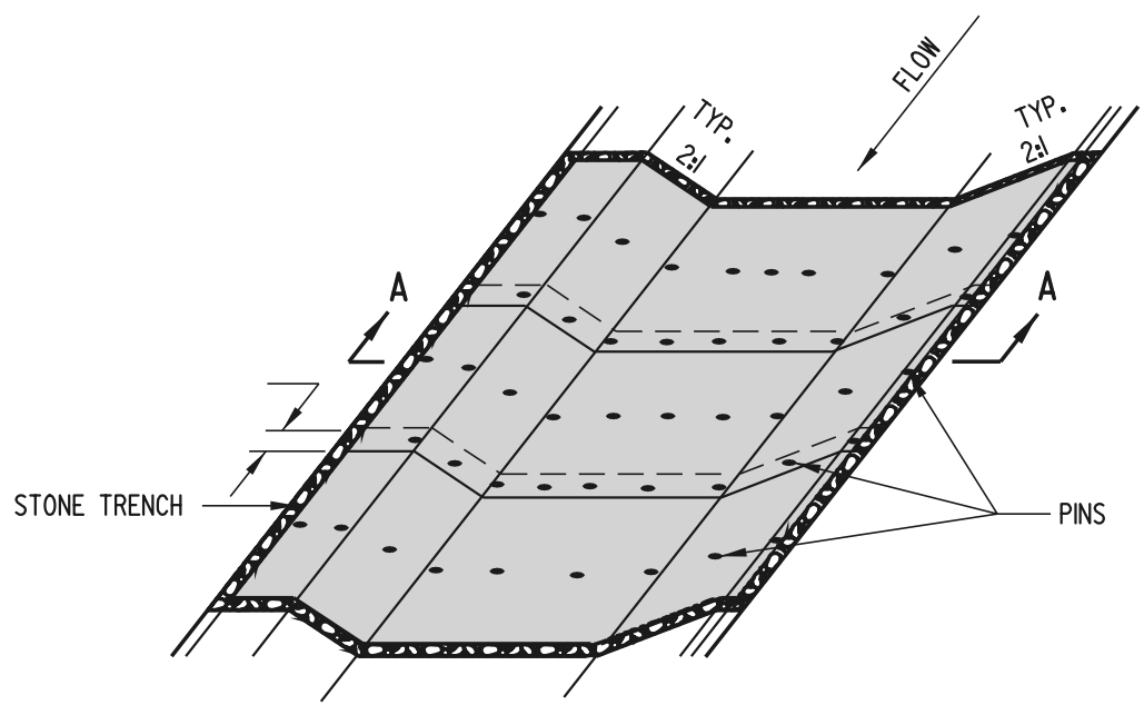
OBLIQUE VIEW
