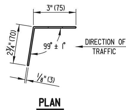
REFLECTORIZED WASHER
