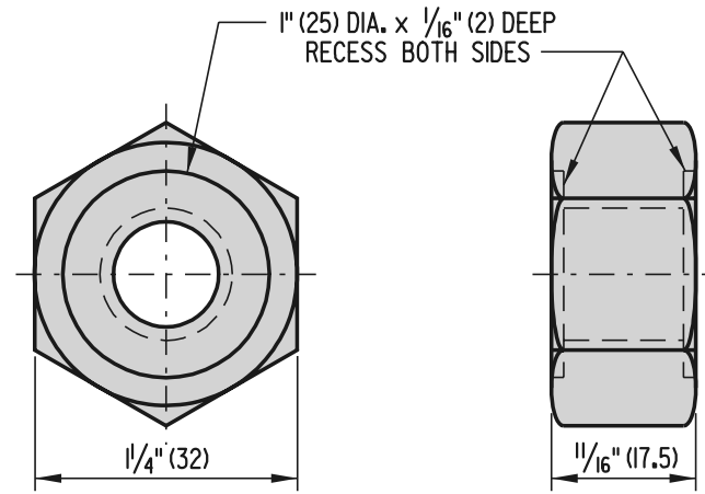
RECESSED NUT (FOR 5/8" (16) GAURDRAIL BOLT)
