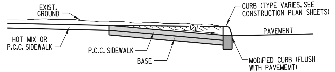
SECTION B-B
