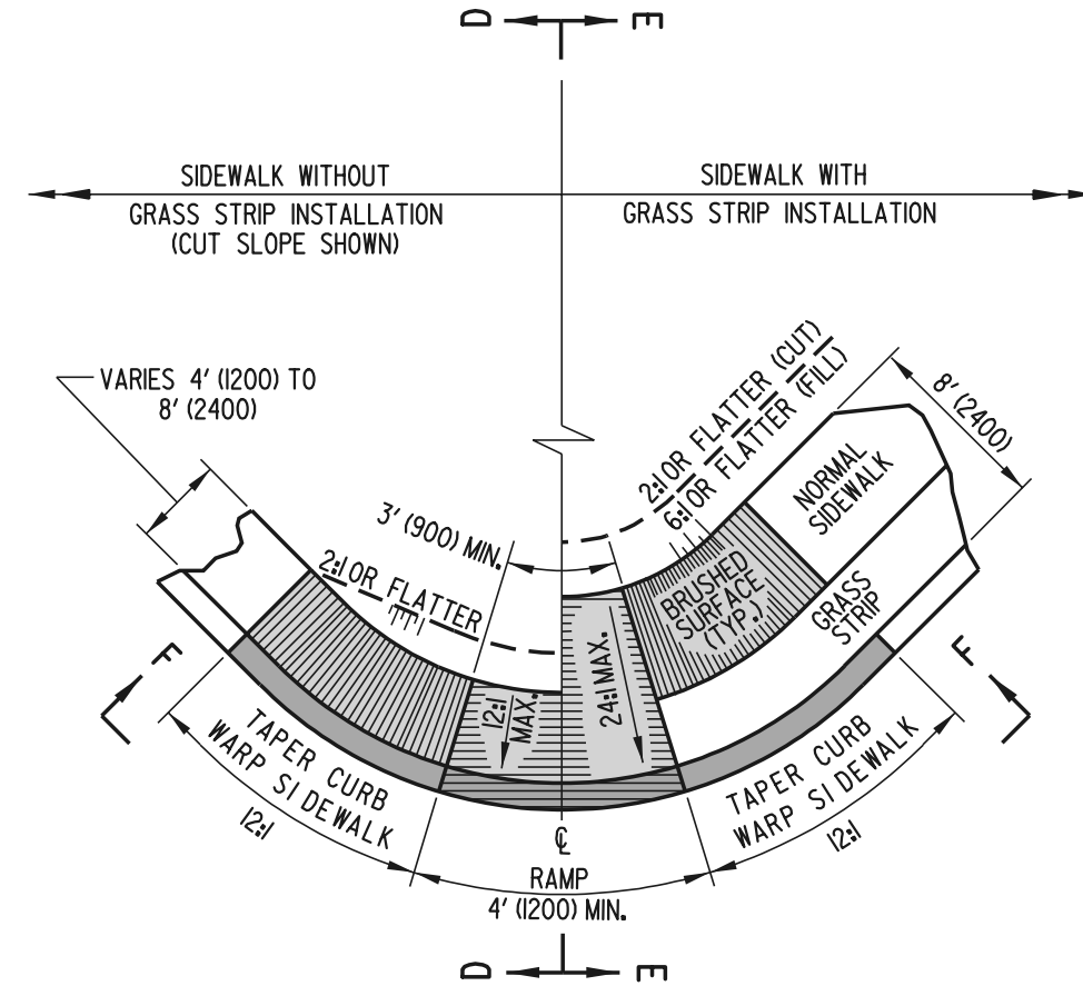
CURB RAMP, TYPE 3
