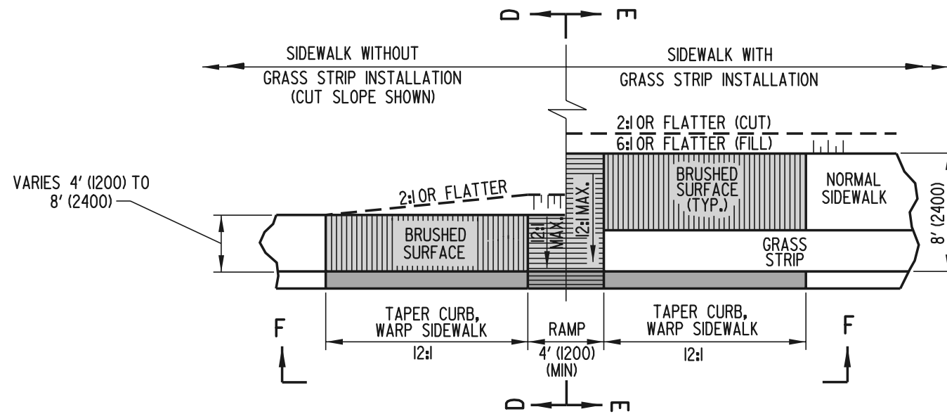
CURB RAMP, TYPE 4
