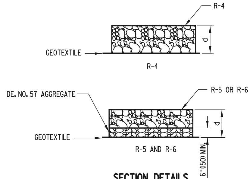
SECTION DETAILS
