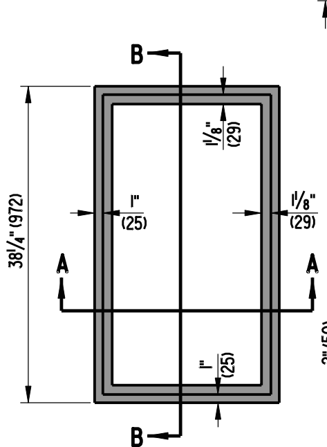
DRAINAGE INLET FRAME
