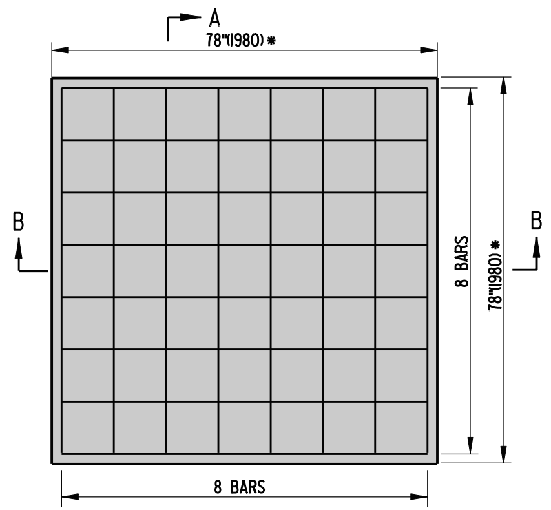
66" (1675) x 66" (1675) JUNCTION BOX
