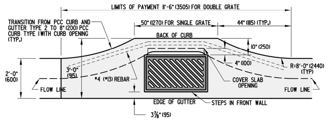
SINGLE GRATE SETUP
