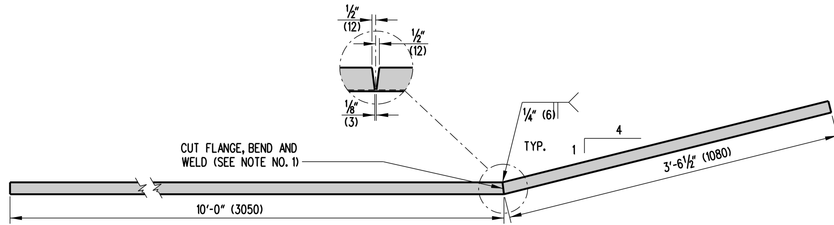
BENT RAIL SCALE: 1"=1'-0"
