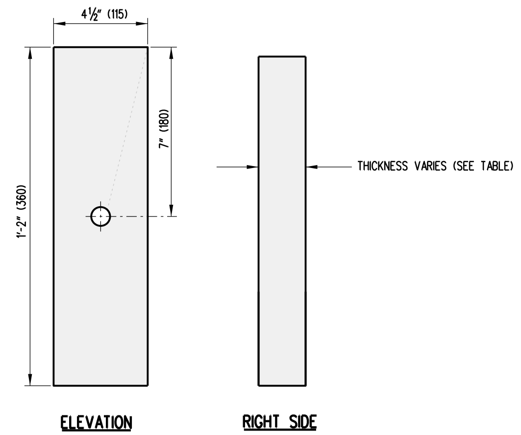
BENT RAIL OFFSET BLOCKS SCALE: 3"=1'-0"
