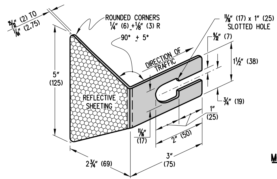
GUARDRAIL DELINEATOR
