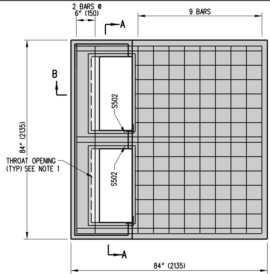
72" (1830) x 72" (1830) INLET
