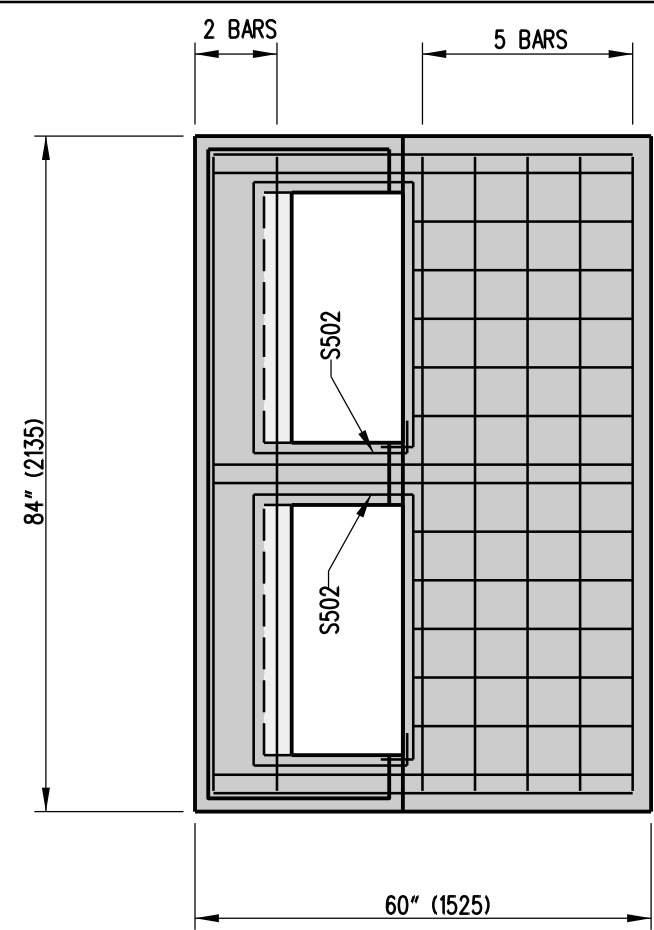
72" (1830) x 48" (1220) INLET
