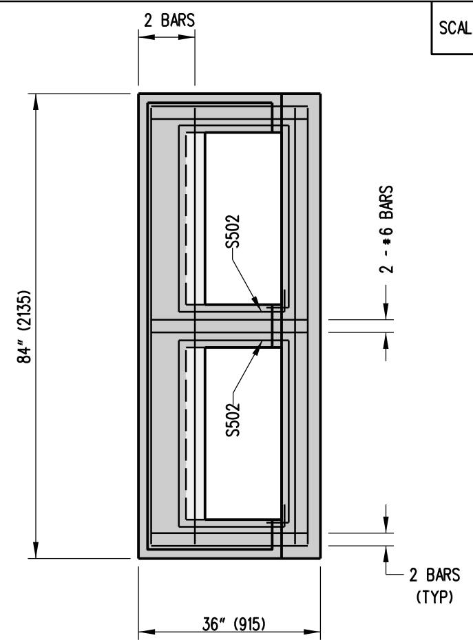
72" (1830) x 24" (610) INLET
