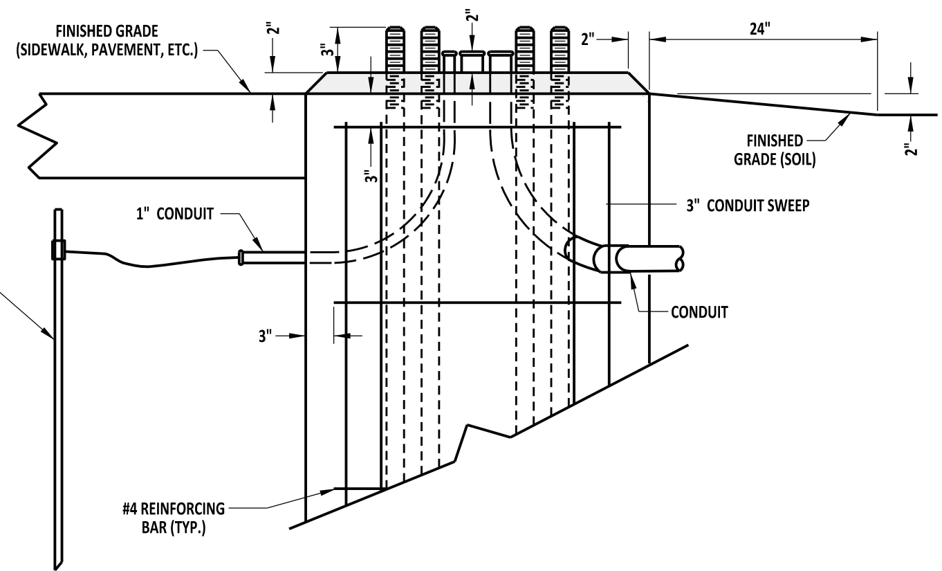
TYPE 7 GROUND ROD TYPICAL
