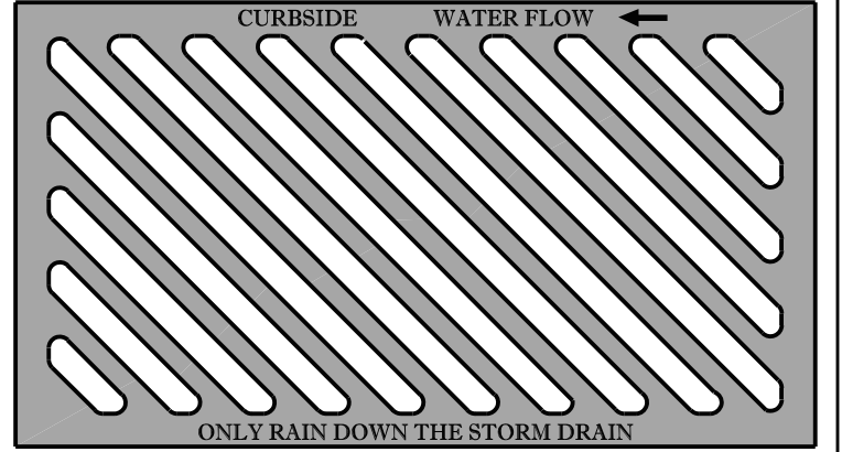
DRAINAGE GRATE LABELING EXAMPLE DETAIL
