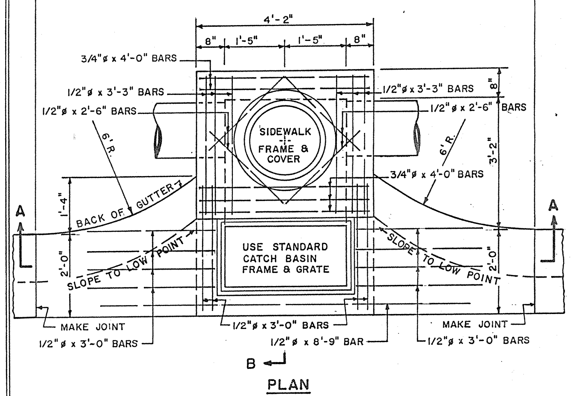
SD-1A CATCH BASIN
