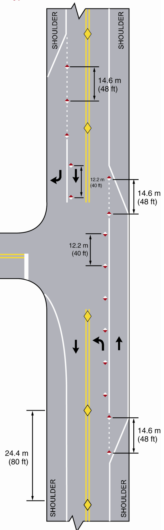
Figure 3B-13G. Example of Raised Pavement Marker (RPM) Application for Deceleration and By-pass Lanes (DelDOT MUTCD Only)
