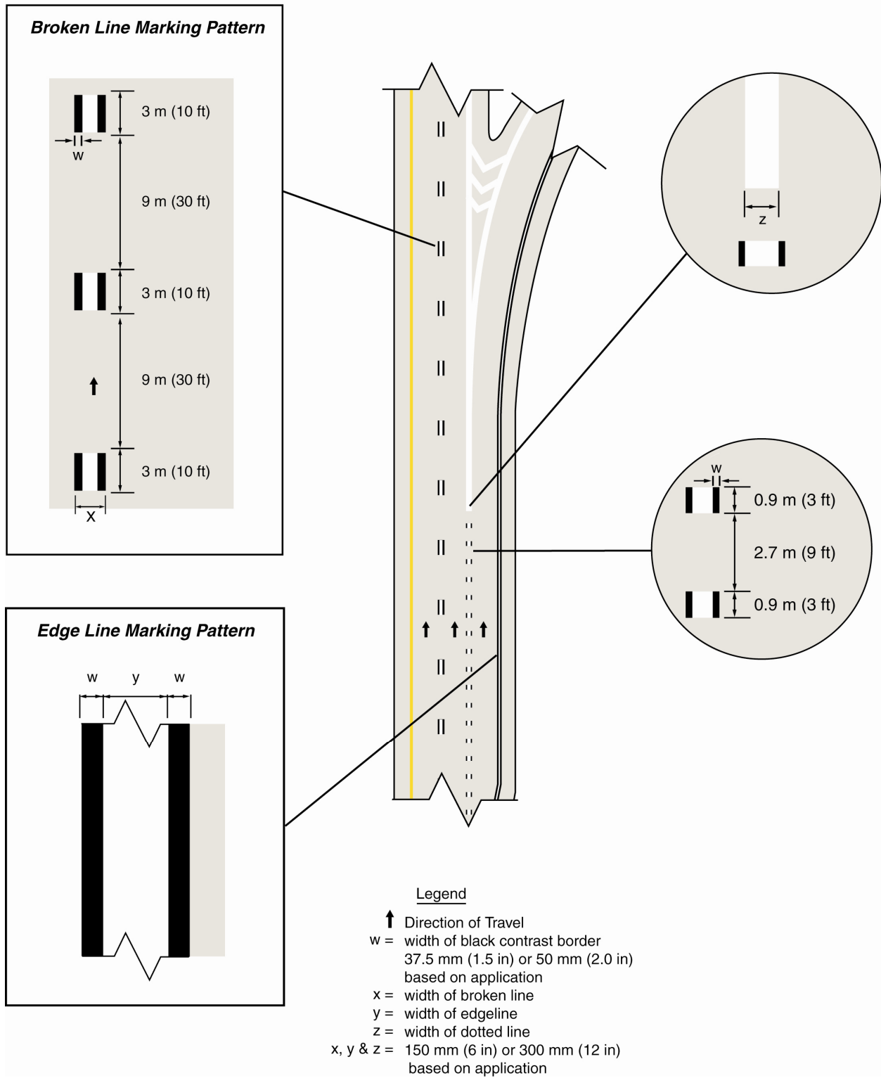
Figure 3A-1A. Black Contrast Marking Patterns on Interstates, Freeways or Expressways (DeIDOT MUTCD Only)
