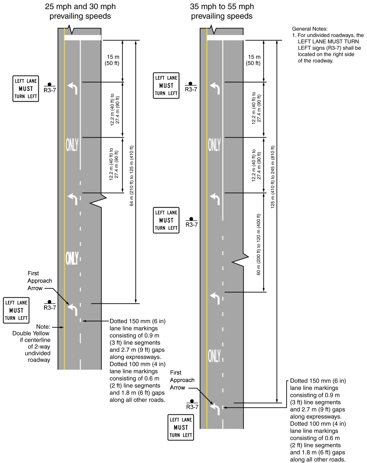
Figure 3B-21A. Examples of Word and Arrow Pavement Markings used in Lane Drop Marking Applications (DeIDOT MUTCD Only)
