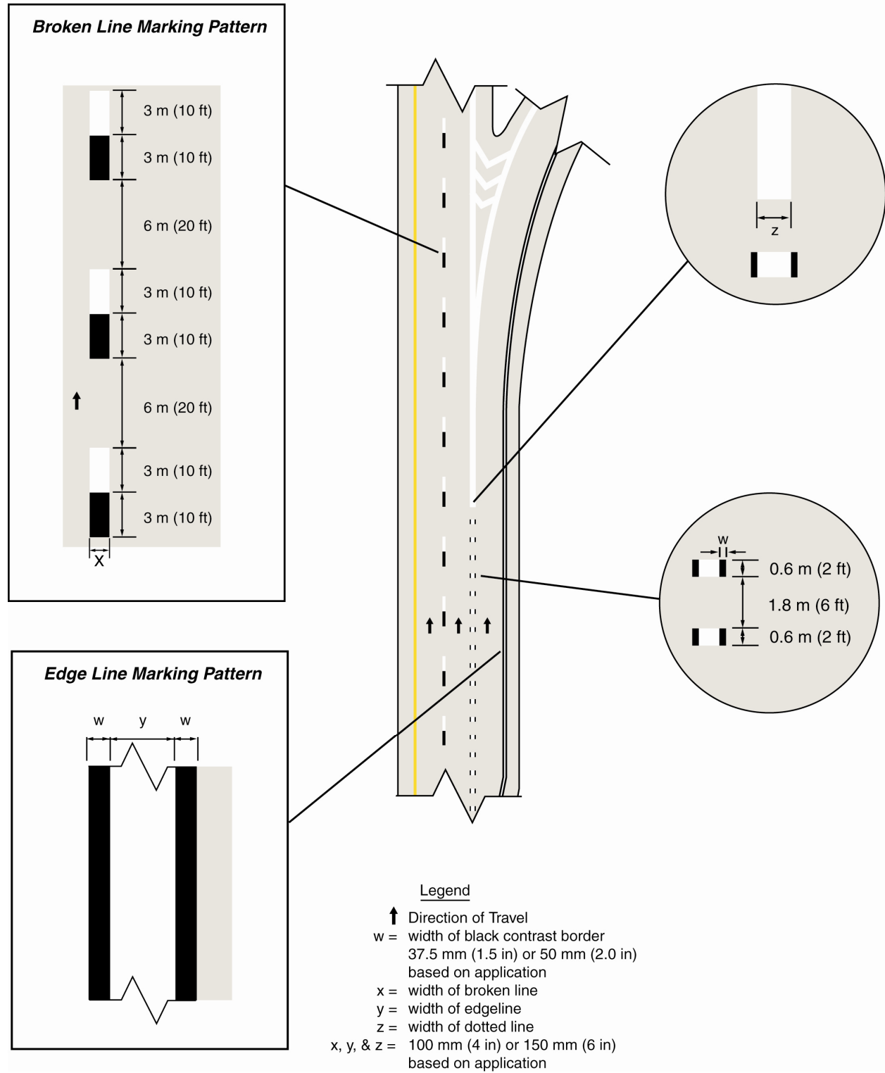
Figure 3A-1B. Black Contrast Marking Patterns on All Other Roads (NON Interstates, Freeways or Expressways) (DelDOT MUTCD Only)
