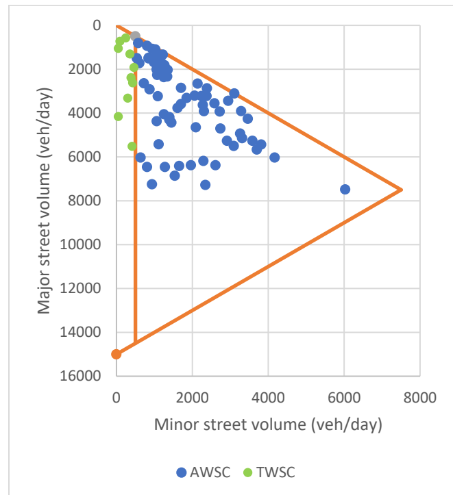
Figure 2. Study Intersections Compared with Optimum Intersection Configuration
