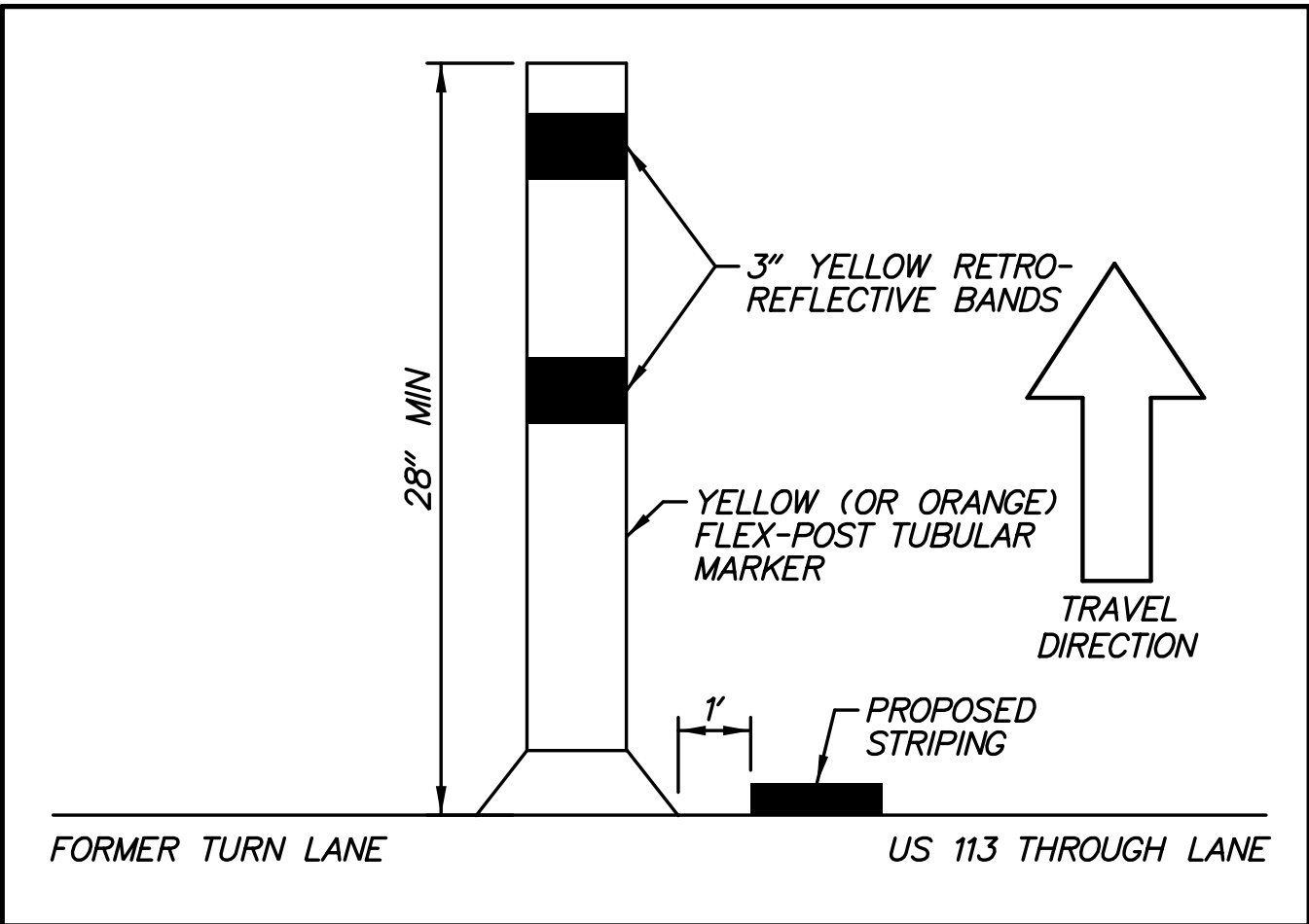
FLEX-POST TUBULAR MARKER INSTALLATION DETAIL SCALE: NONE
